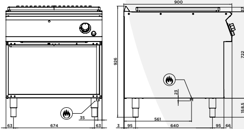
EM94TPG
