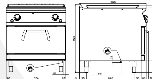
EM94TFG
